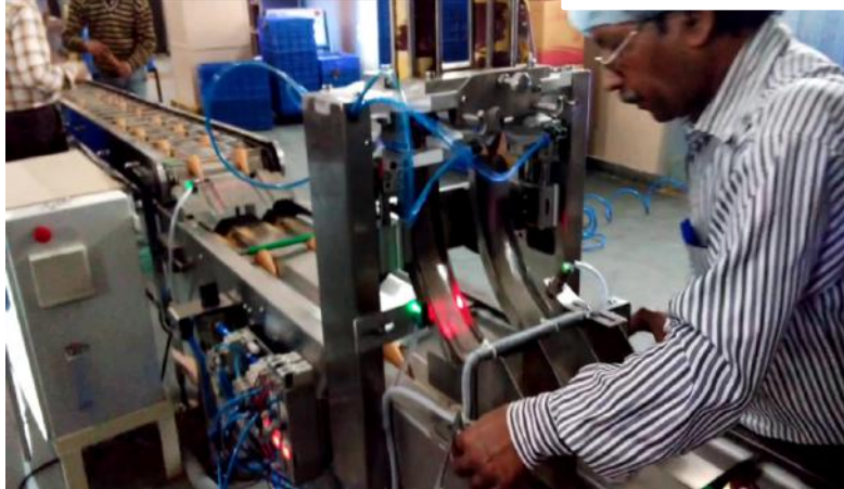
SPM Cone Sleeve System
